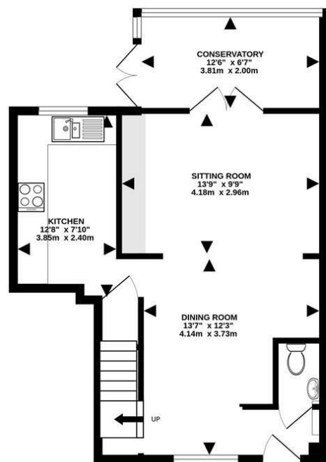
GROUND FLOOR 502 sq.ft. (46.6 sq.m.) approx.
